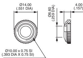
KNURLED CAP NUT (std for 10600)
