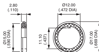
SEALING WASHER
