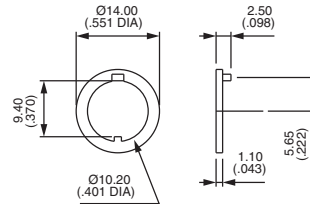
LOCKING RING
