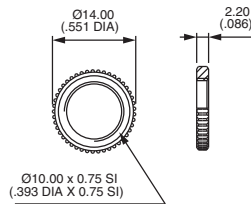
KNURLED NUT (std for 10400)
