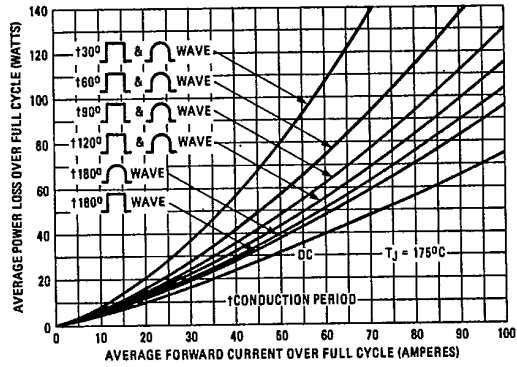
Fig. 10 - Maximum Forward Power Loss Vs. Forward Current
