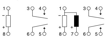
Schematic (Bottom view) <2 Form A> Single side stable (Deenergized condition) 2 coil latching (Reset condition)
