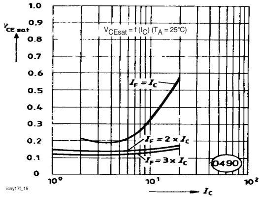
Figure 15. Saturation Voltage vs. Collector Current and Modulation Depth CNY17F-4
