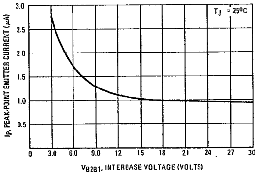
FIGURE 8 - EFFECT OF VOLTAGE
