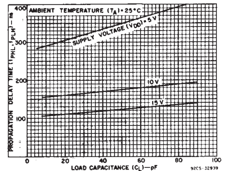
Fig. 8—Typical propagation delay time as a function of load capacitance (Astable, Astable to Q, Q-bar).
