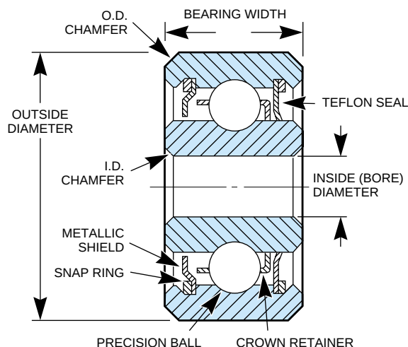
Cross section view of ball bearing
