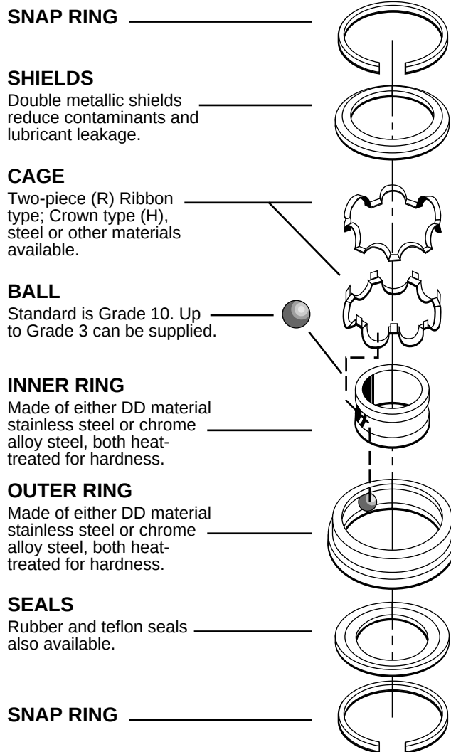
Exploded view of ball bearing
