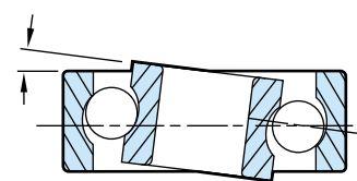
Figure 5. Free angle of the bearing.
