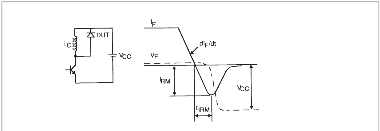
Fig. 14: Turn-off switching characteristics (with series inductance).
