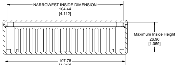
SECTION C-C
