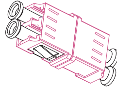
LC violet body (SC simplex footprint)
