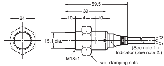
E2A-M18KN10-WP-□□/E2A-S18KN10-WP-□
