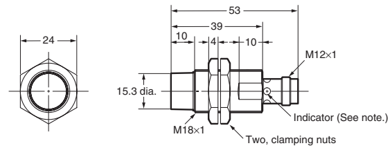
E2A-M18KN10-M1-□□/E2A-S18KN10-M1-□
