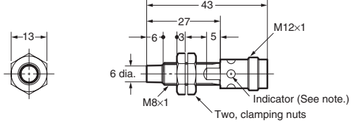
E2A-S08KN02-M1-□□
