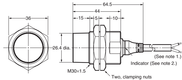
E2A-M30KN18-WP-□□/E2A-S30KN18-WP-□
