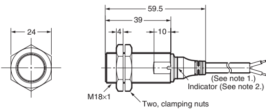
E2A-M18KS05-WP-□□/E2A-S18KS05-WP-□
