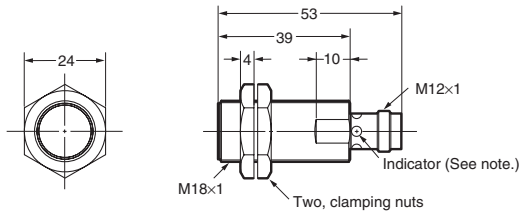
E2A-M18KS05-M1-□□/E2A-S18KS05-M1-□
