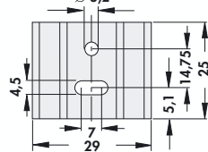
SK 145 25 TO 220
