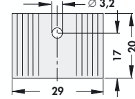
SK 09 20 TO 220
