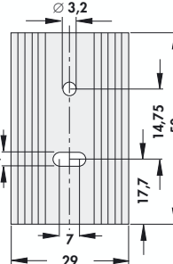
SK 09 50 TO 220
