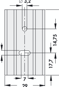
SK 145 50 TO 220
