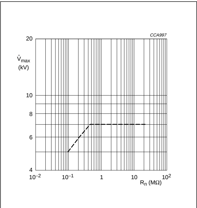
Fig.2 Maximum allowed peak pulse voltage in accordance with “IEC 60065 chapter 14.1”; 50 discharges from a 1 nF capacitor charged to \hat{V}_{max} ; 12 discharges/minute (drift \Delta R/R \leq 1\% ).
