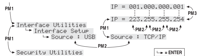
(C) Detalle del menú UTILITY: Interface Utilities
