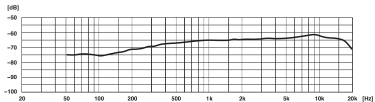
Frequenzgang Frequency response
