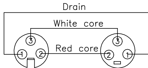
Wiring Method
