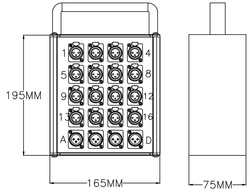
Stage box
