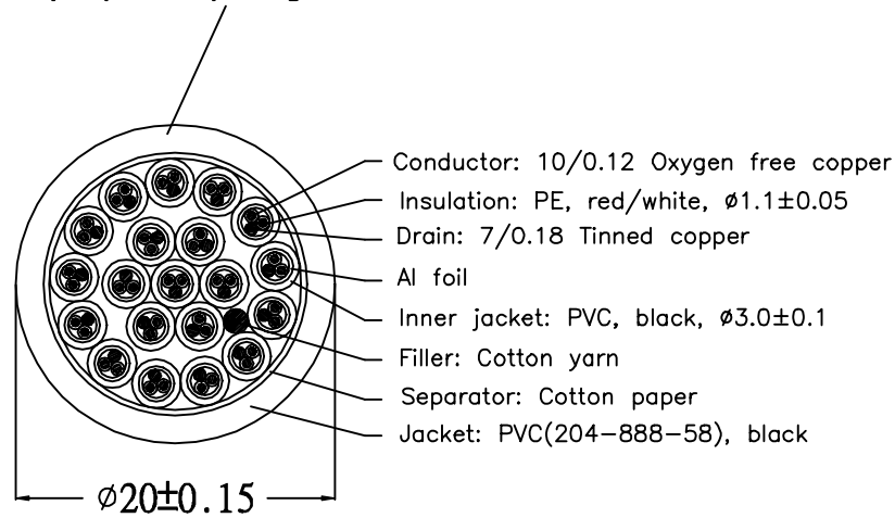
Cable Construction
