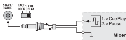
Fig. 10 Fader start via control pulse
