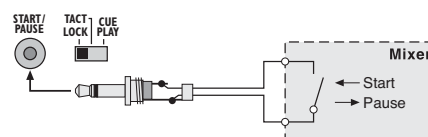
Fig. 8 Fader start via on/off switch
