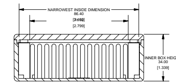
SECTION D-D SCALE 3/4
