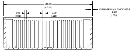
SECTION A-A SCALE 3 / 4
