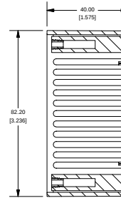
SECTION B-B SCALE 3 / 4
