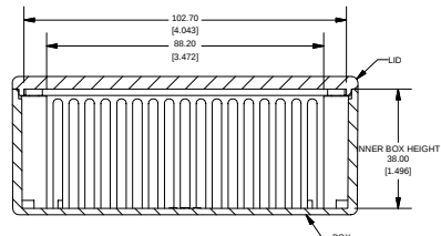
SECTION C-C SCALE 3 / 4
