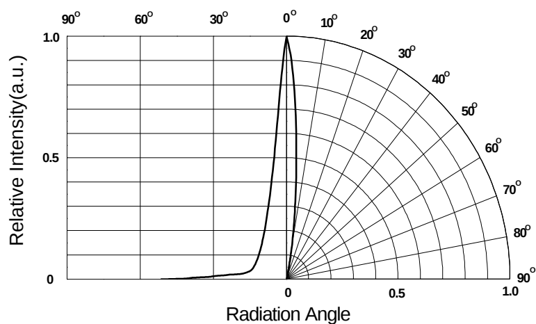
Radiation Characteristics
