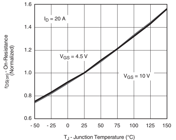
I_D = 20 A V_{GS} = 4.5 V V_{GS} = 10 V T_J - Junction Temperature (°C) On-Resistance vs. Junction Temperature
