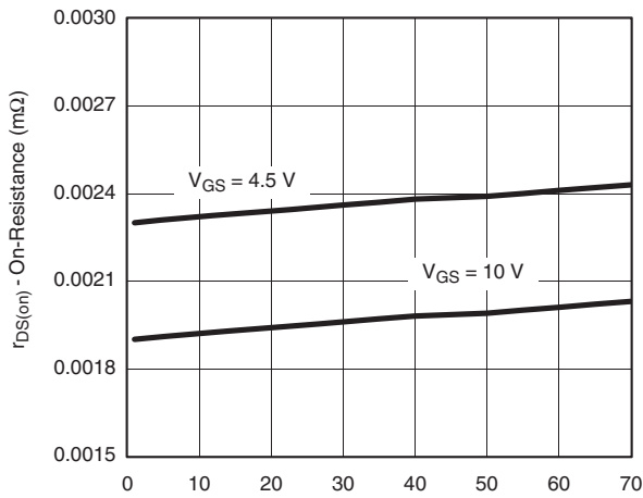
V_{GS} = 4.5 V V_{GS} = 10 V On-Resistance vs. Drain Current and Gate Voltage
