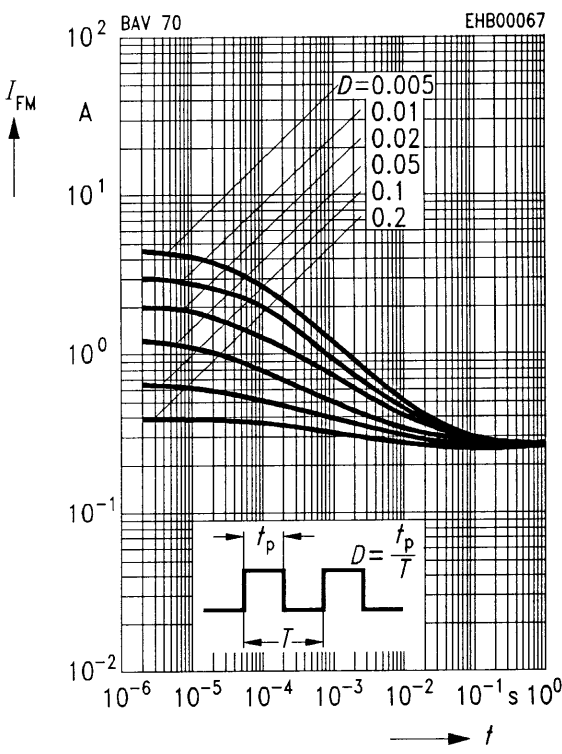
Peak forward current I_{FM} = f(t) T_A = 25^\circ\text{C}
