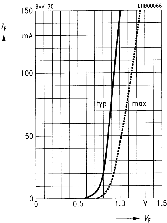
Forward current I_F = f(V_F) T_A = 25^\circ\text{C}
