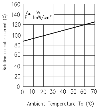
Fig. 3 Relative Collector Current vs. Ambient Temperature
