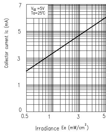
Fig.4 Collector Current vs. Irradiance
