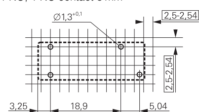
1 NO, 1 NC contact 5 mm
