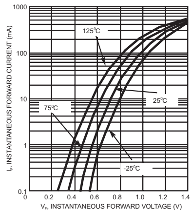
FIG.5- FORWARD CHARACTERISTIC CURVE
