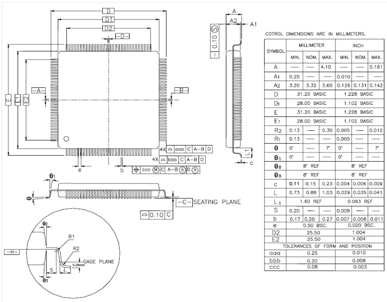
Figure 42-2. 208-lead TQFP Package Drawing
