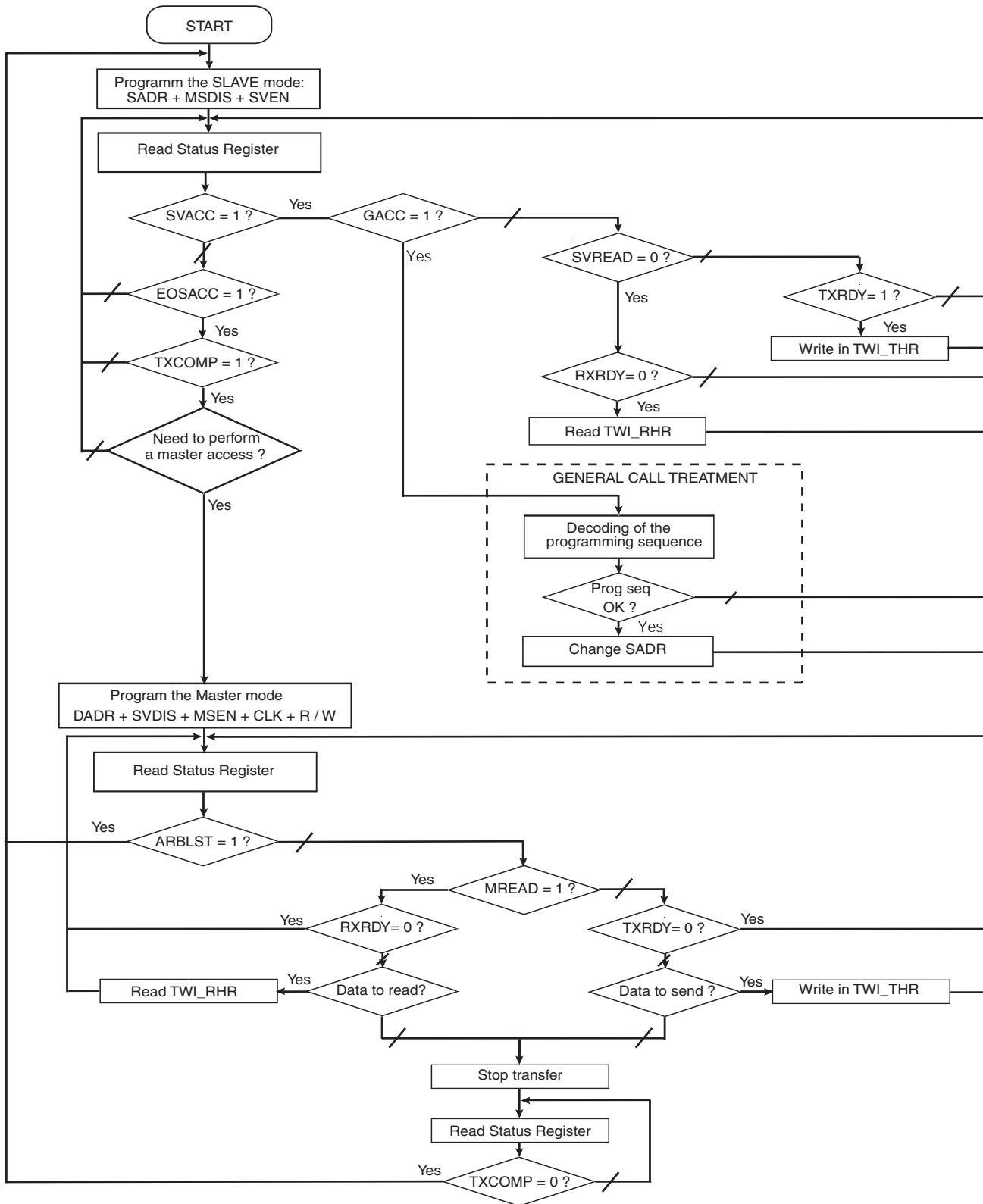
Figure 31-22. Multi-master Flowchart
