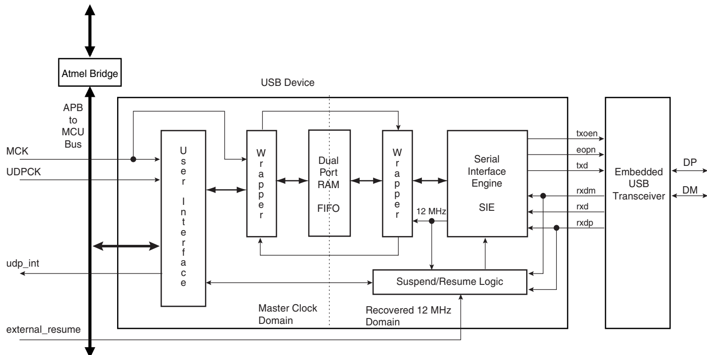
Figure 38-1. Block Diagram
