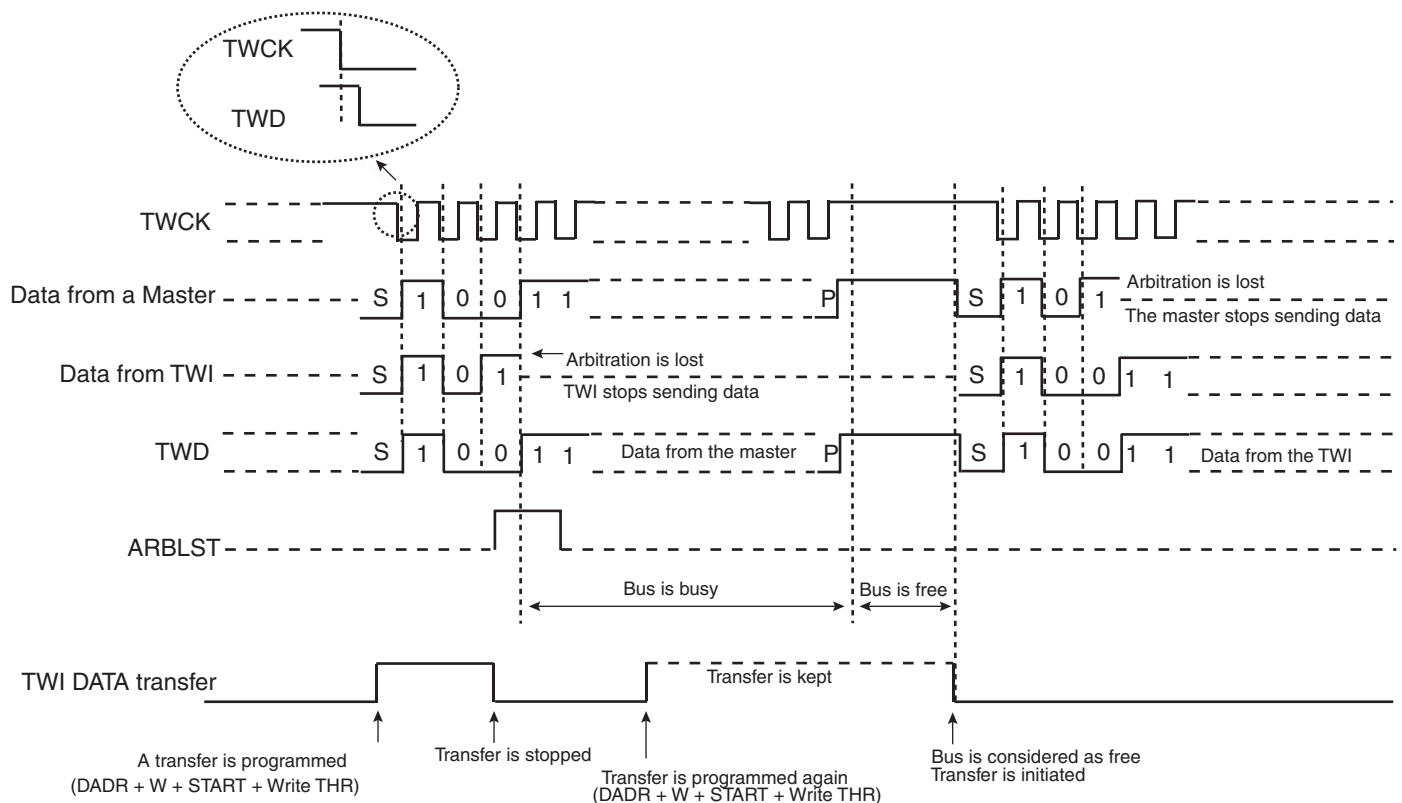
Figure 31-21. Arbitration Cases
