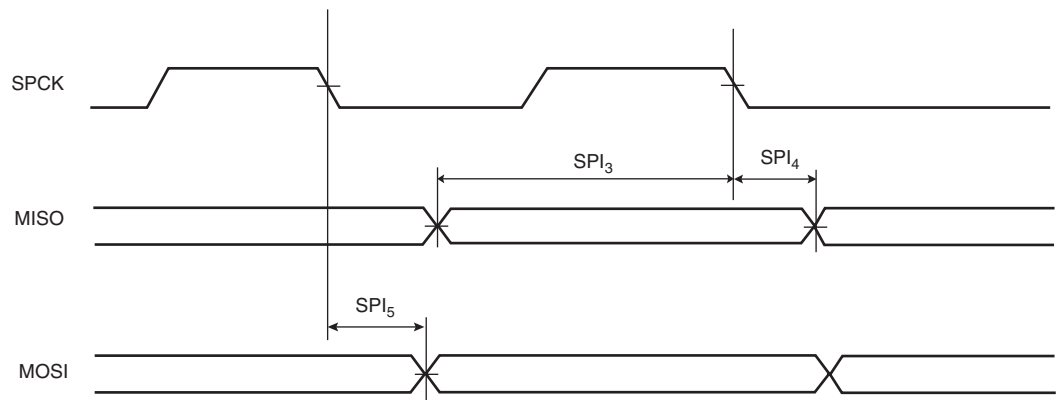
Figure 41-7. SPI Master Mode with (CPOL=0 and NCPHA=1) or (CPOL=1 and NCPHA=0)
