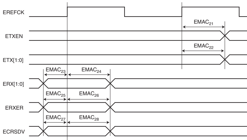
Figure 41-5. EMAC RMII Mode
