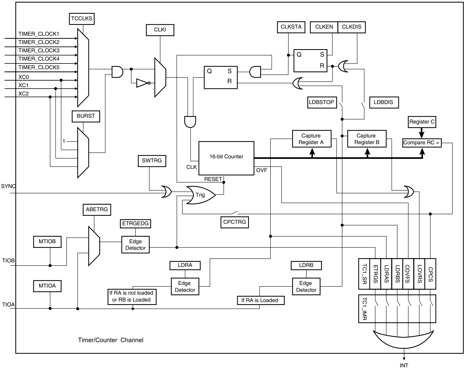
Figure 34-5. Capture Mode
