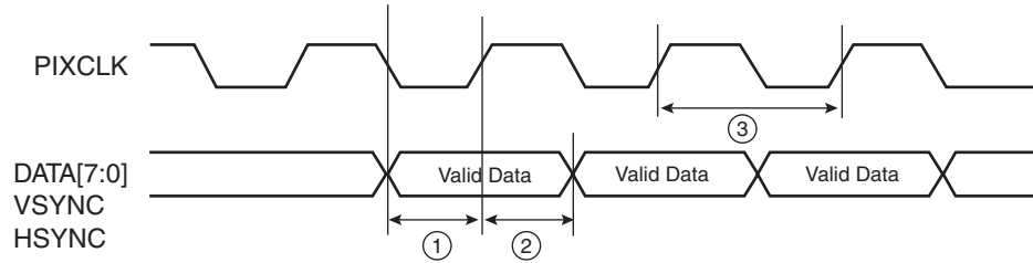
Figure 41-10. ISI Timing Diagram
