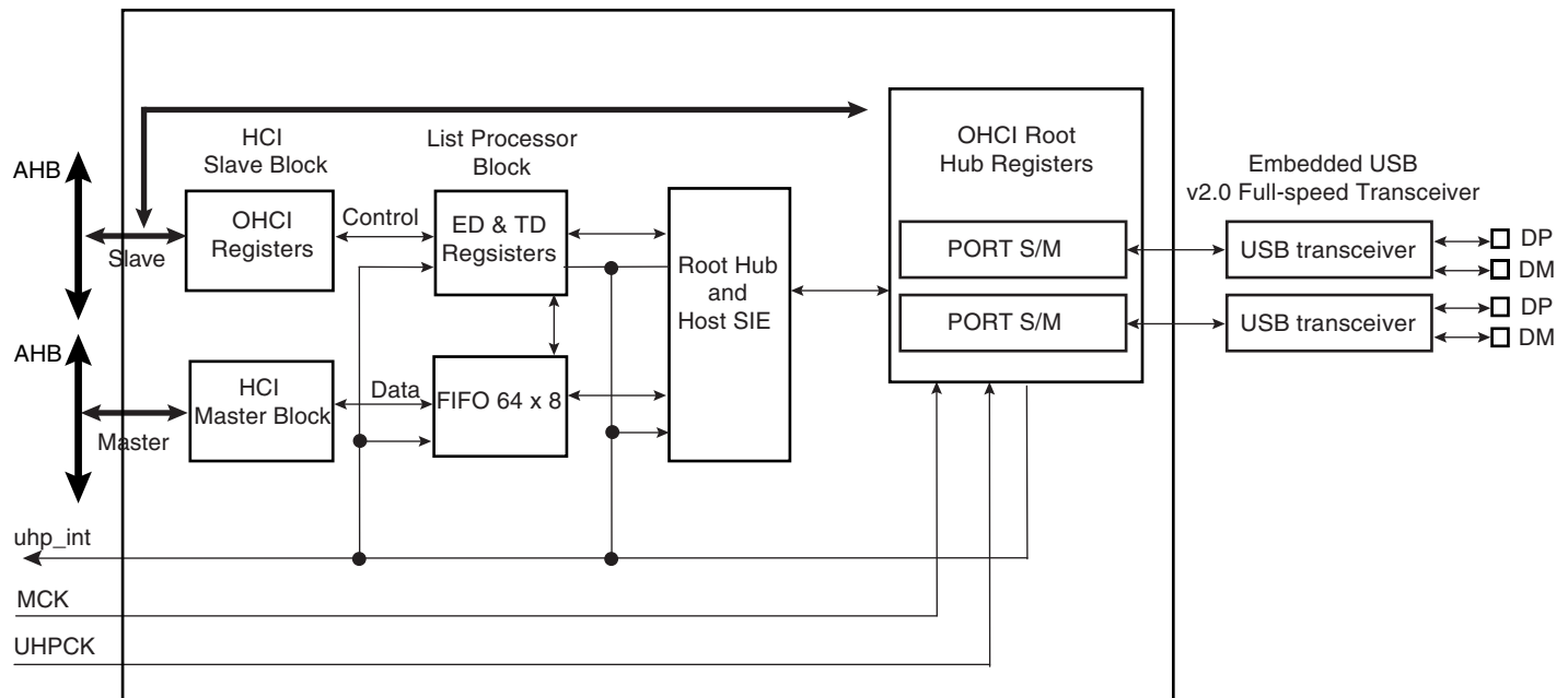
Figure 37-1. Block Diagram
