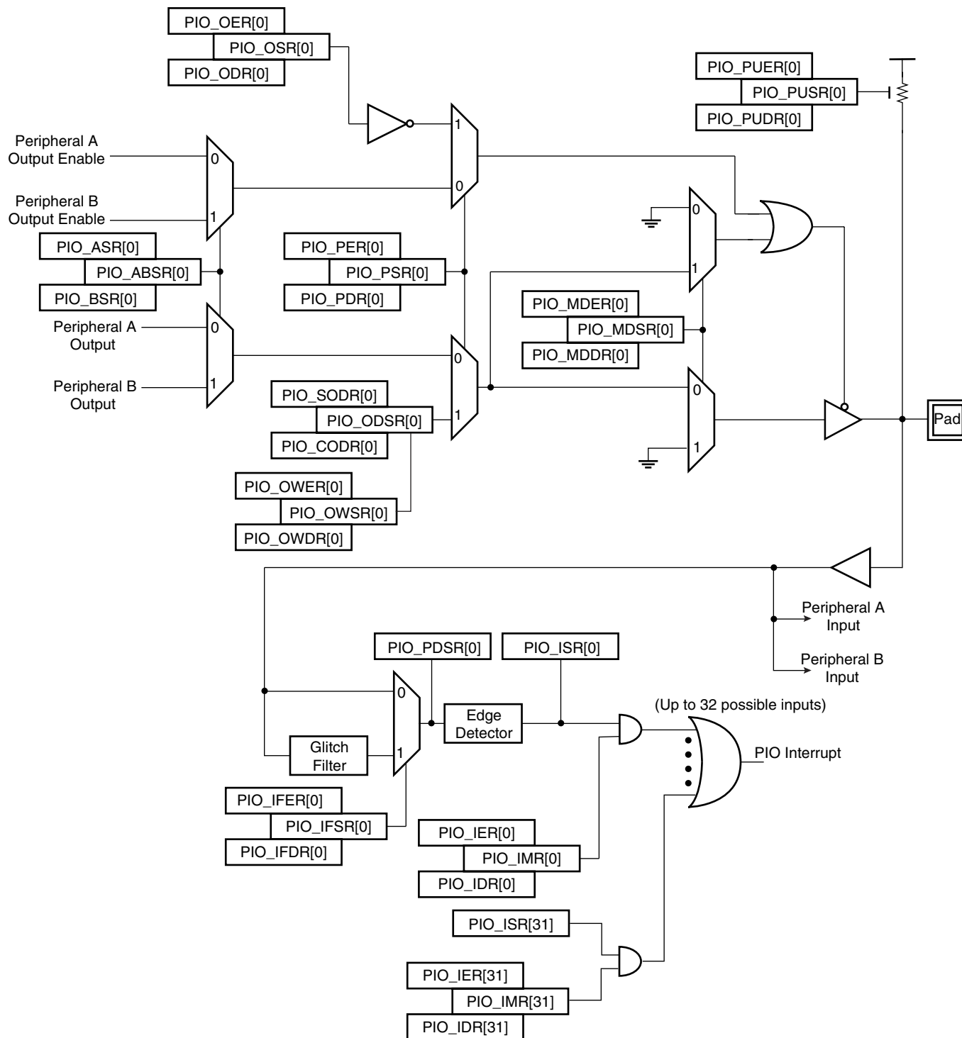
Figure 30-3. I/O Line Control Logic
