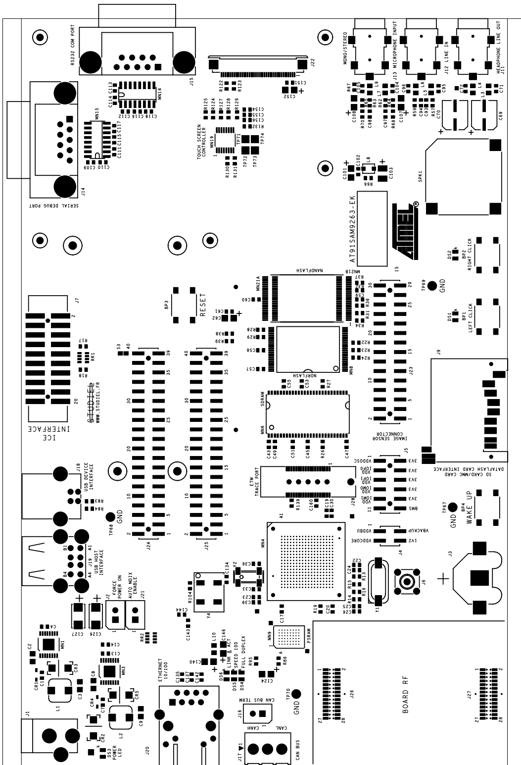
Figure 2-1. AT91SAM9263-EK Layout - Top View
