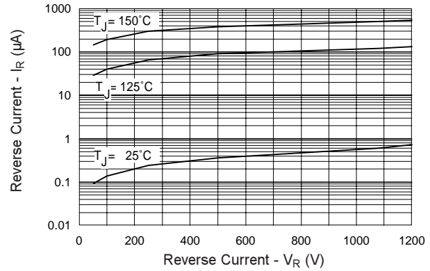
Fig. 2 - Typical Reverse Current vs. Reverse Voltage
