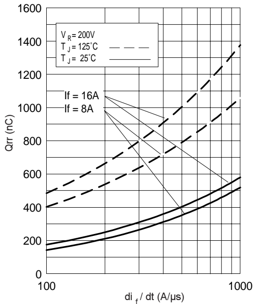
Fig. 7 - Typical Stored Charge vs. di_f/dt , (per Leg)
