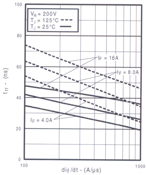
Fig. 14 - Typical Reverse Recovery vs. di/dt
