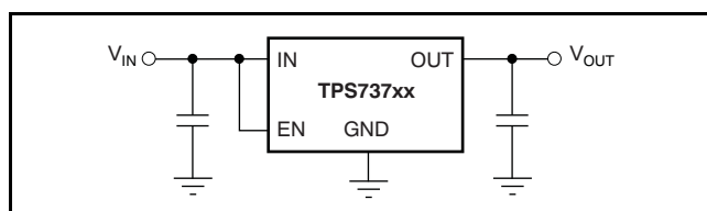
Figure 31. Typical Application Circuit for Fixed-Voltage Versions
