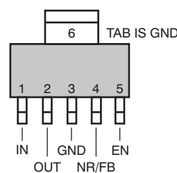
DCQ PACKAGE SOT223 (TOP VIEW)
