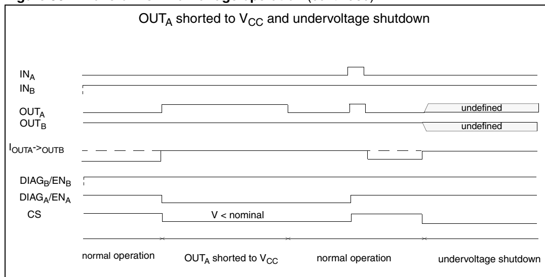
Figure 36. Waveforms in full bridge operation (continued)
