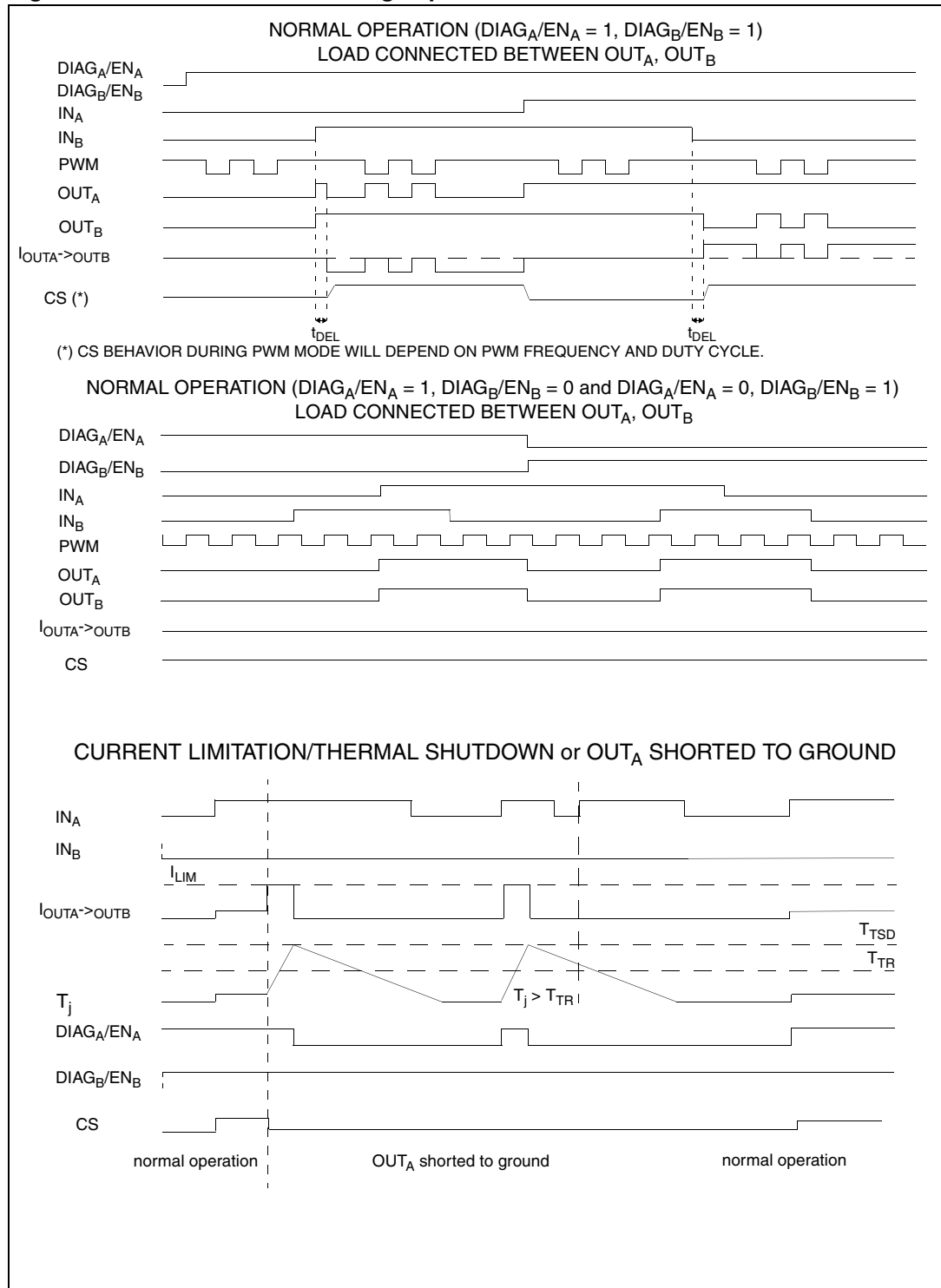
Figure 35. Waveforms in full bridge operation
