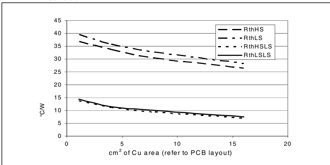
Figure 39. Auto and mutual R_{thj-amb} vs PCB copper area in open box free air condition
