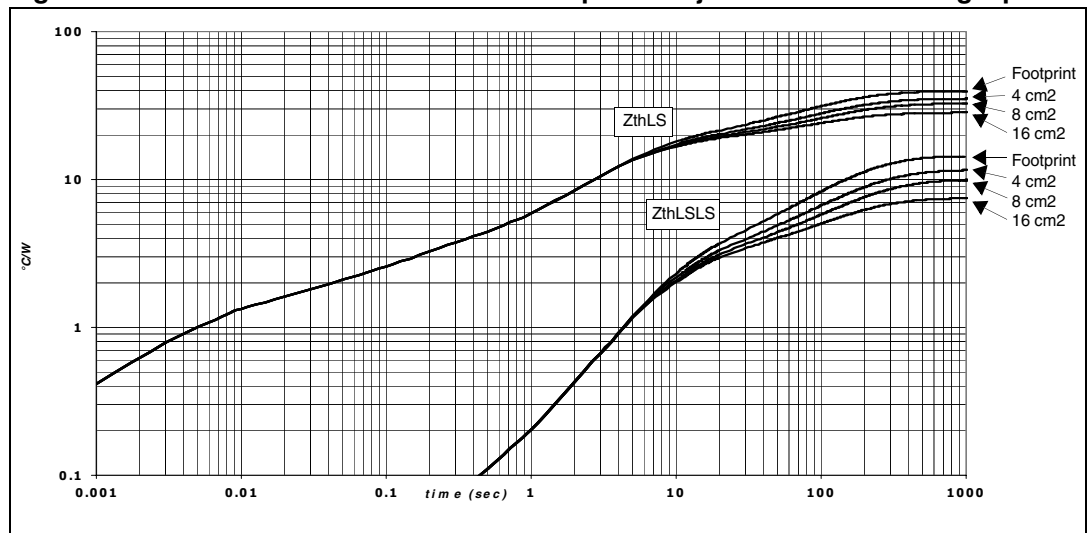
Figure 41. MultiPowerSO-30 LSD thermal impedance junction ambient single pulse
