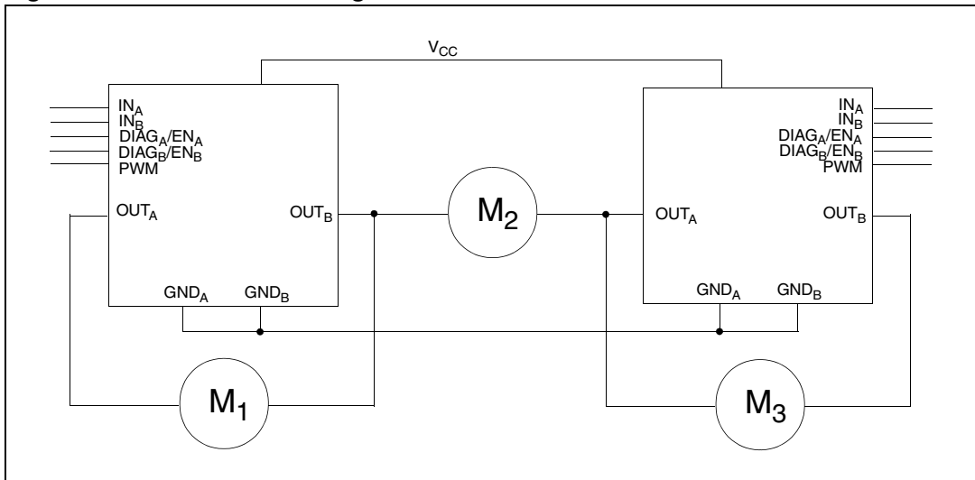
Figure 34. Multi-motors configuration
