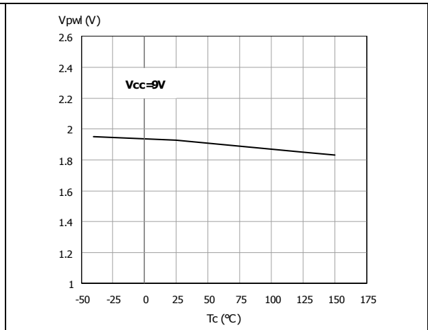
Figure 21. PWM low level voltage
