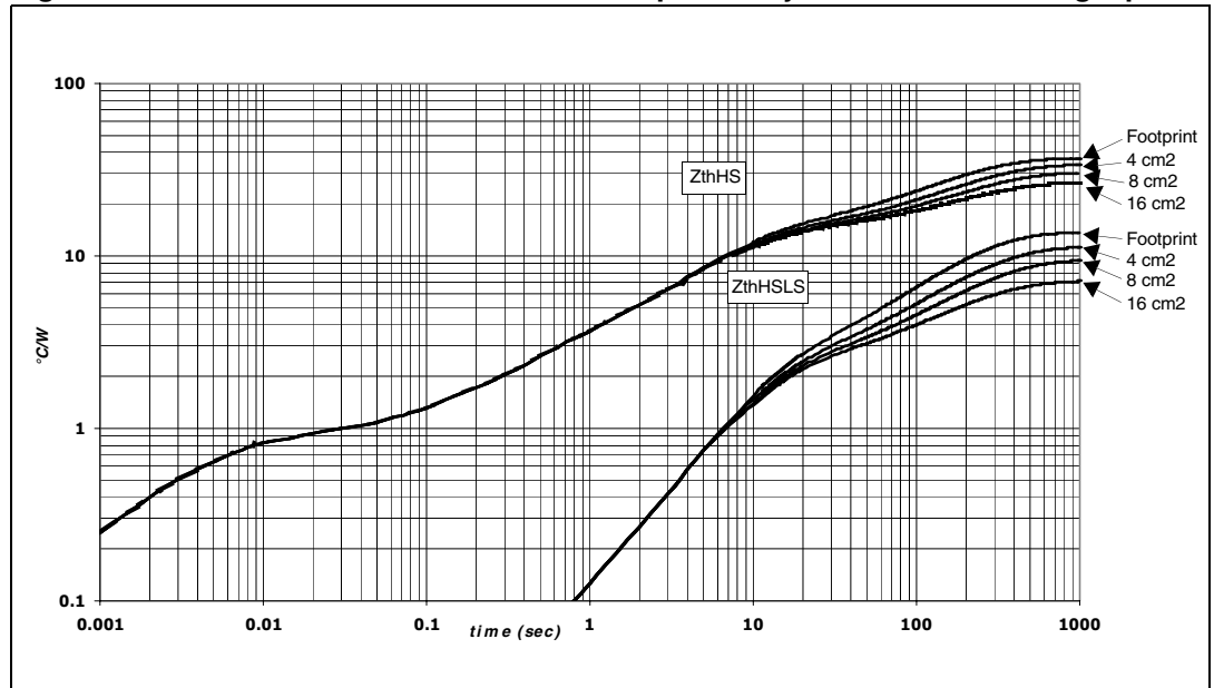
Figure 40. MultiPowerSO-30 HSD thermal impedance junction ambient single pulse
