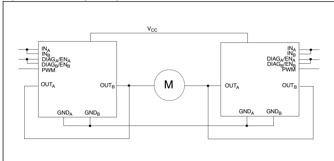
Figure 33. Half-bridge configuration
