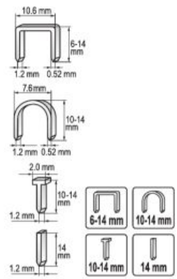
YATO YT-7001 12/24
