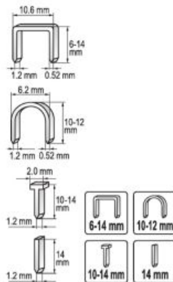
YATO YT-7000 12/24
