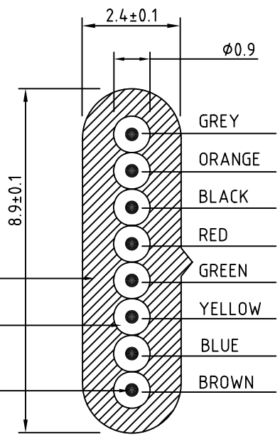
SECTION K-K
