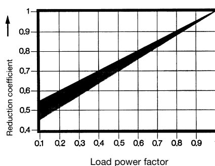
2 Reduction of expected life against load power factor cos \varphi
