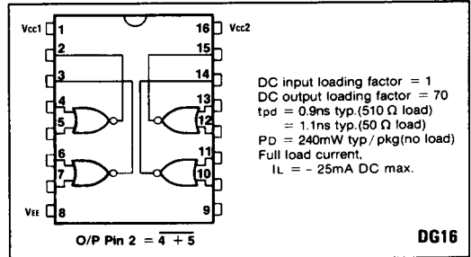
Fig.1 Logic diagram
