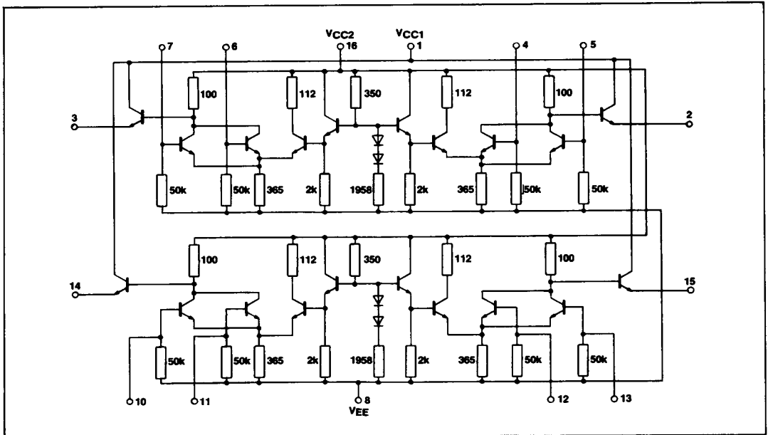
Fig.2 Circuit diagram
