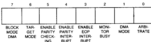
Figure 5. Mode Register
