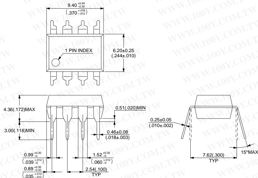
8-pin Plastic DIP (DIP-8P-M01)
